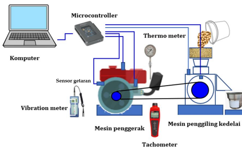
Gambar 4 . Set-up aparatus penelitian.
