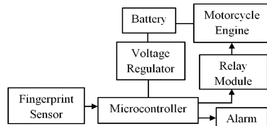
Figure 1. Block diagram representing proposed fingerprint-based key system architecture
