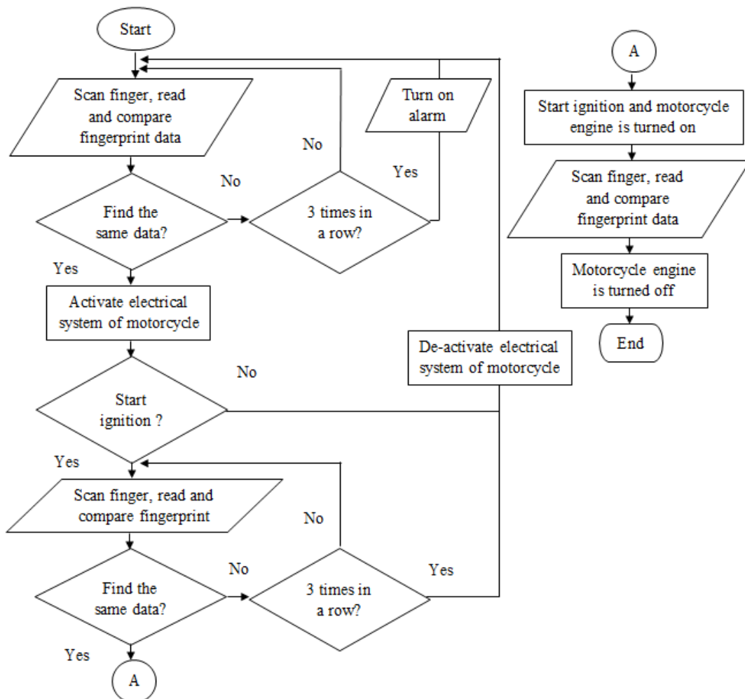
Figure 6. Flowchart of overall computational steps of microcontroller
