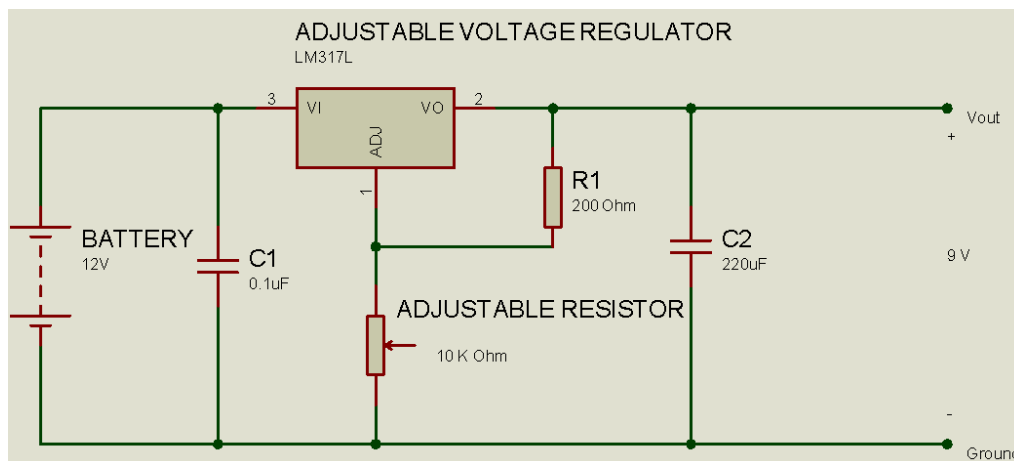
Figure 2. Voltage regulator circuit
