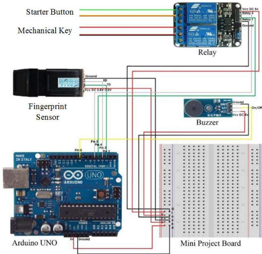
Figure 3. Wiring diagram of main components
