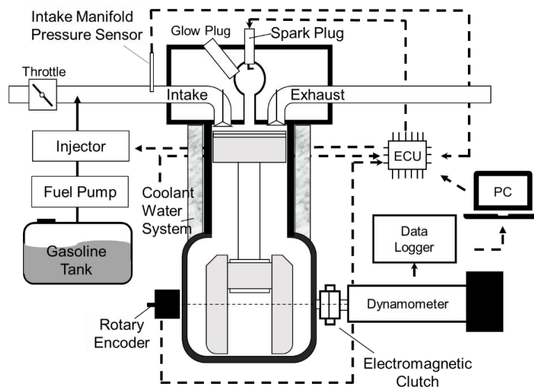
Figure 1. Schematic of the experiment setup.
