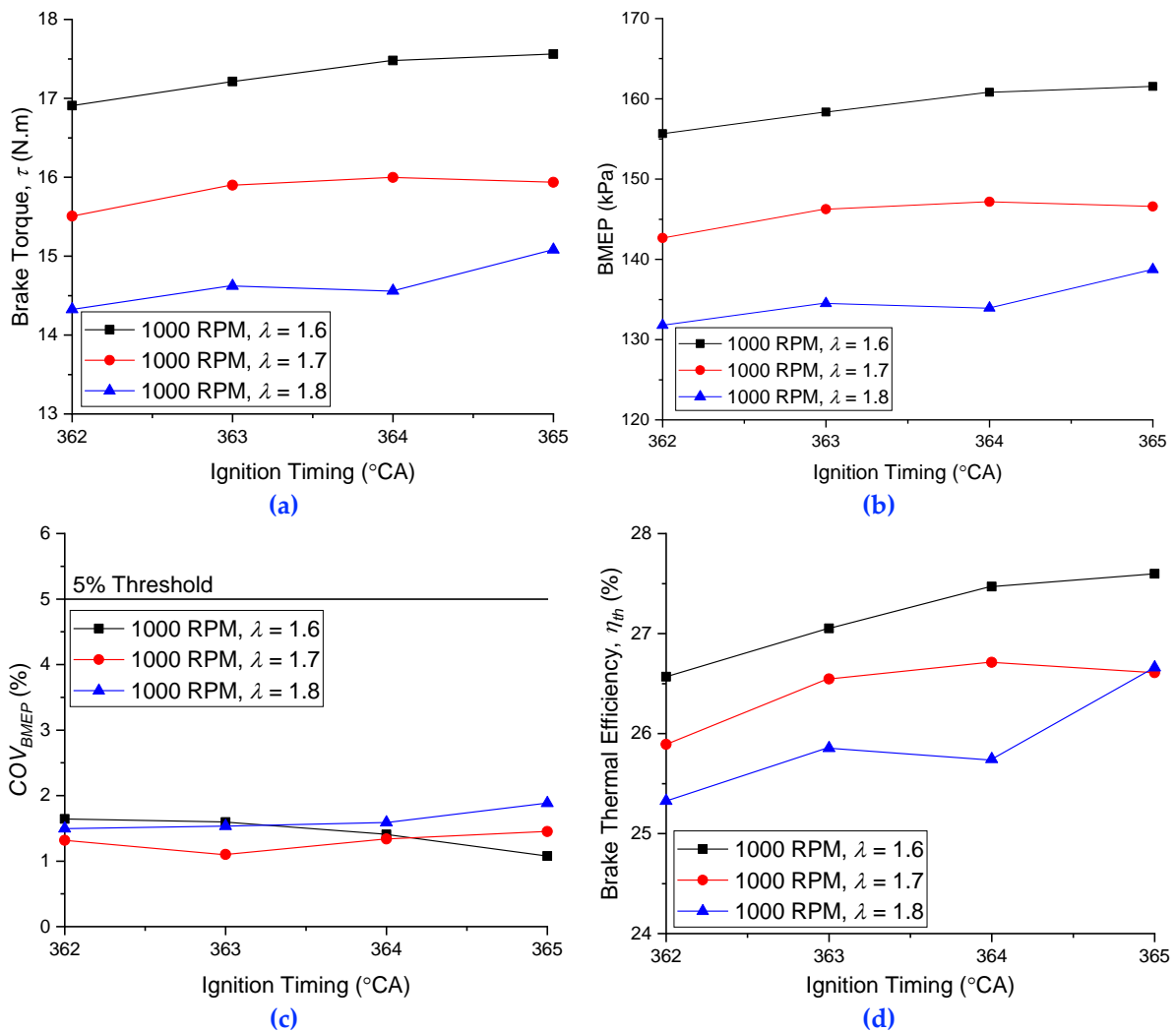
Figure 3. Engine performances of lean iso-octane/air mixtures for the second set of experiment. The investigated parameters include (a) brake torque, (b) BMEP, (c) COV of the BMEP, and (d) brake thermal efficiency.
