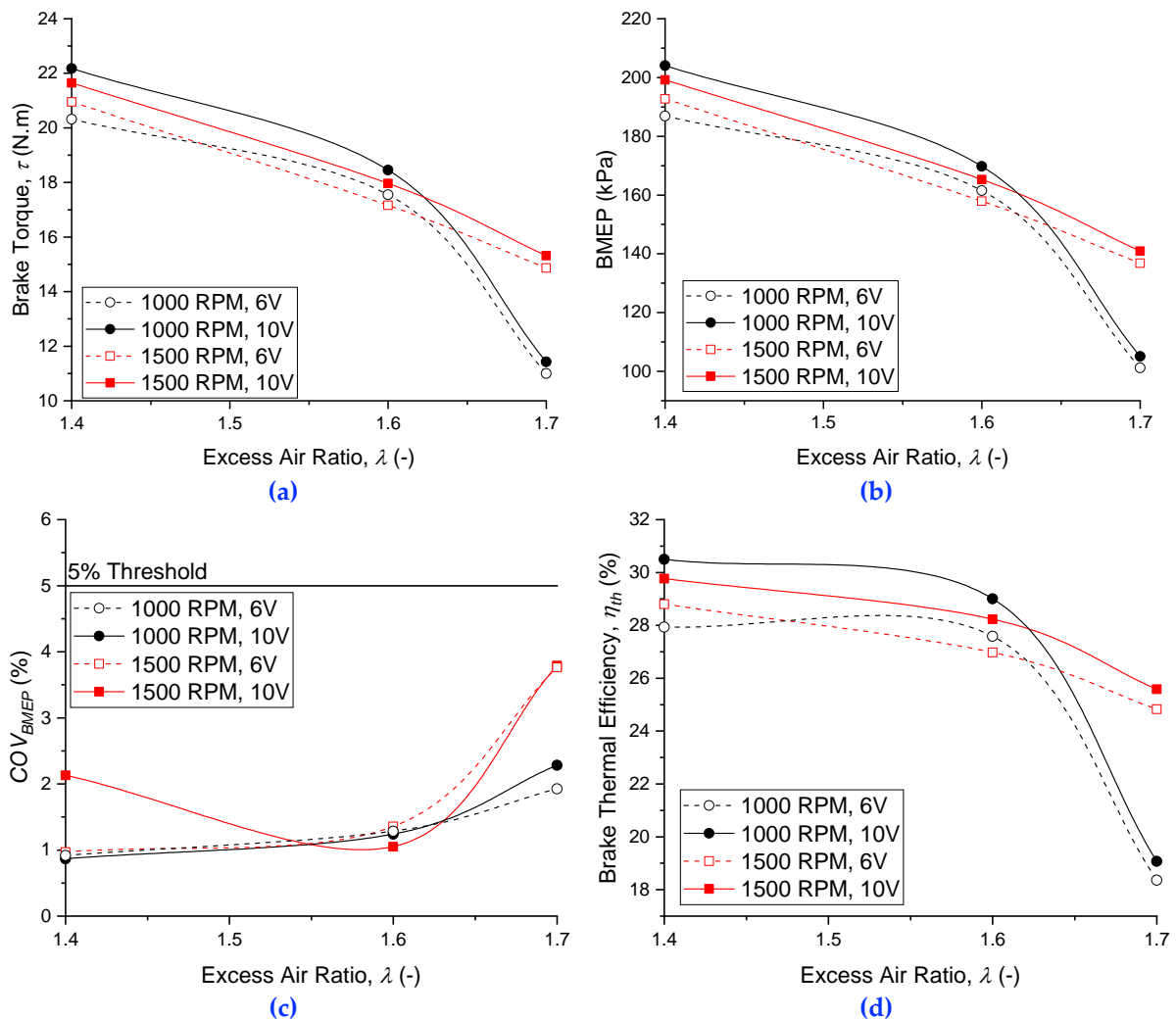
Figure 2. Engine performances of lean iso-octane/air mixtures for the first set of experiment. The investigated parameters include (a) brake torque, (b) BMEP, (c) COV_{BMEP} , and (d) brake thermal efficiency.
