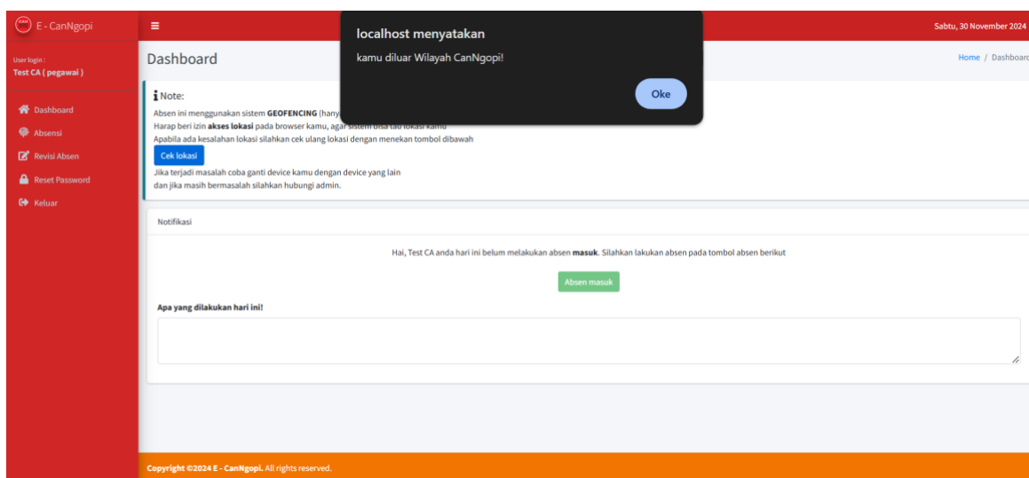
Gambar 11. Absensi Geofencing
